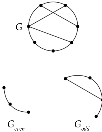
Figure 1: G_{even} and G_{odd}
