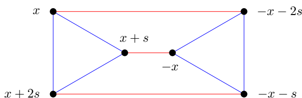
Figure 1: A component of a distinct link graph.
