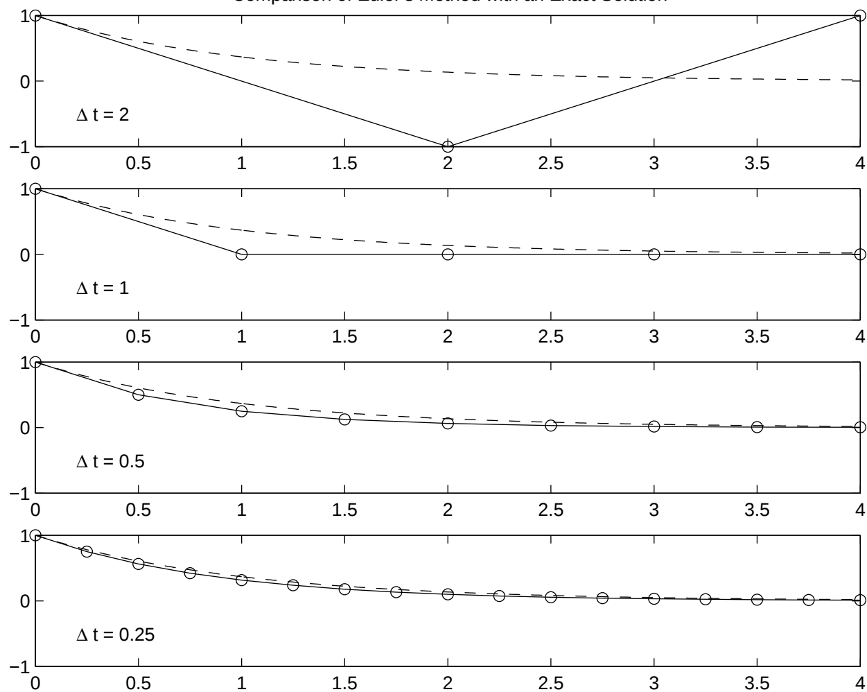
Comparison of Euler's Method with an Exact Solution
